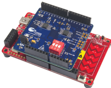
CY15FRAMKIT-001 kit with PSoC 4 Pioneer Kit
